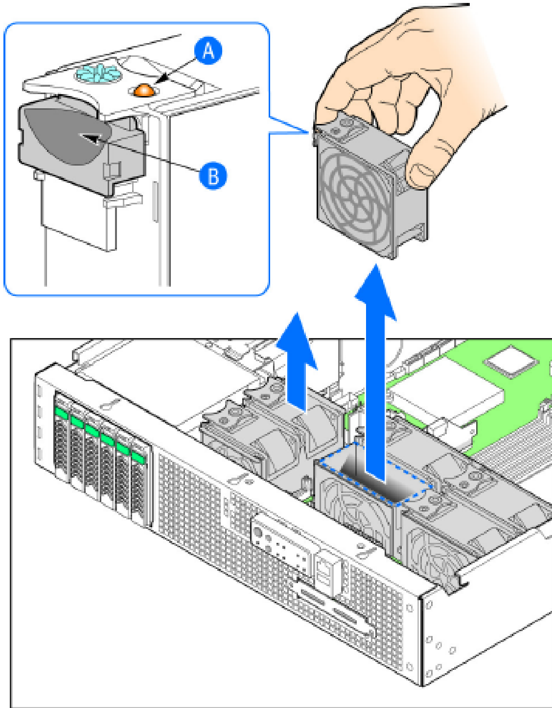
FIGURE 321 Replacing a system fan
