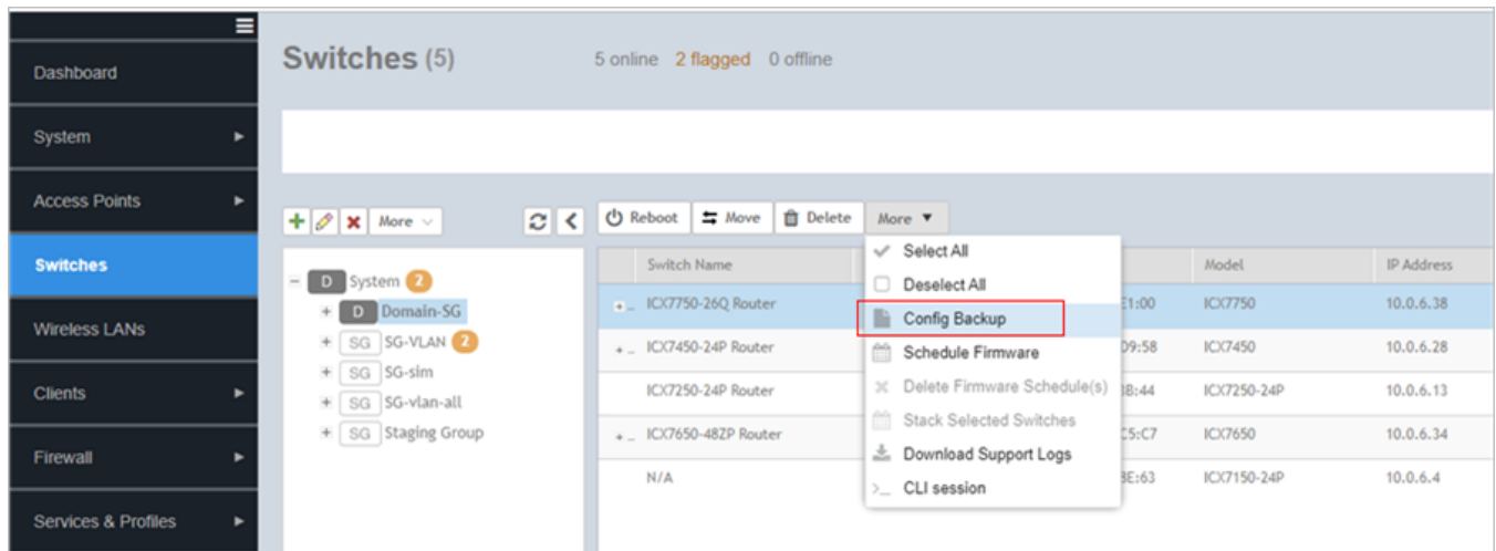
FIGURE 79 Configuring Backup
