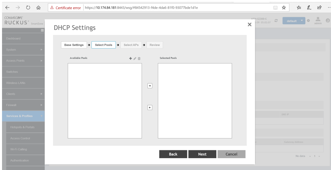
FIGURE 249 Selecting Pools
