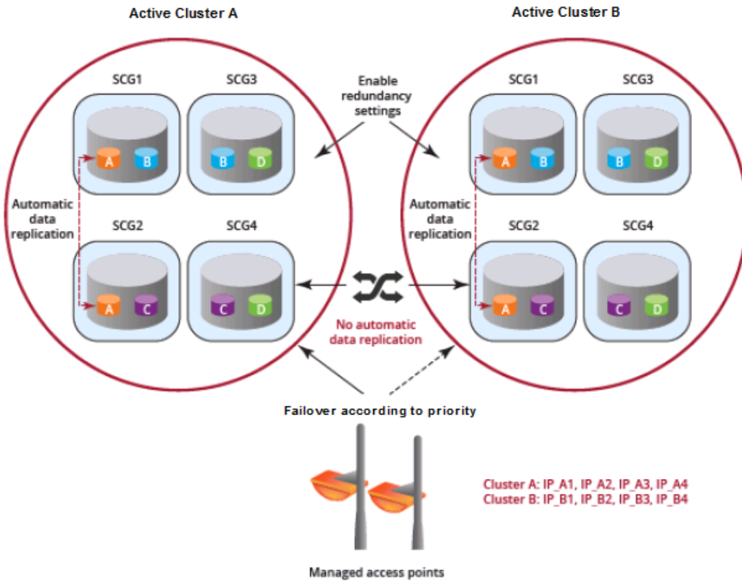
FIGURE 67 Cluster Redundancy for Active-Active Mode
