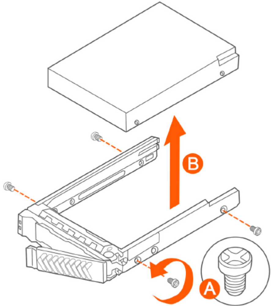
FIGURE 317 Removing the hard drive
